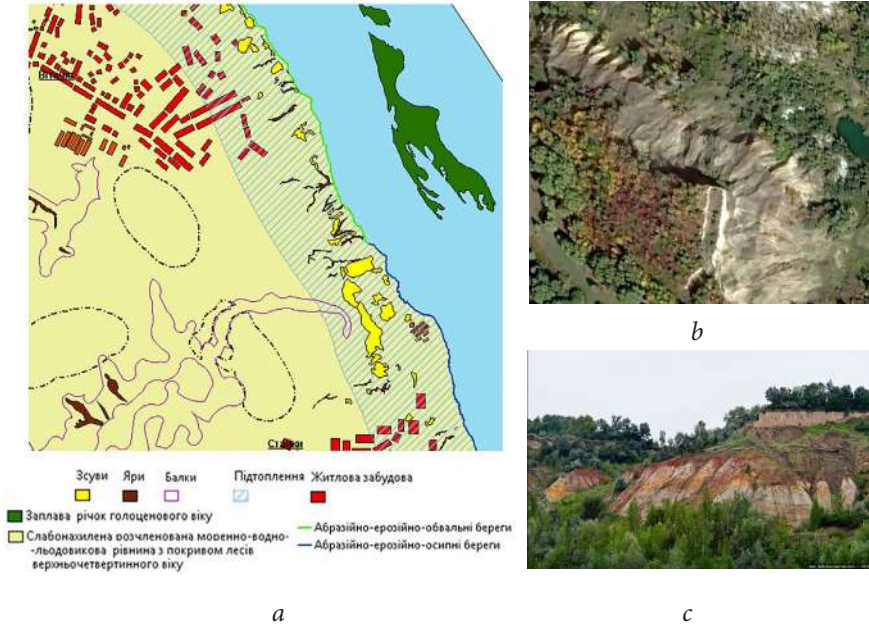
Fig. 4.26. Study of landslide processes on the right bank of the Kaniv Reservoir within the boundaries of Kyiv Region, as exemplified by the area of Vytachiv-Stayky: a — fragment of the map; b — appearance in the satellite image caused by quarrying operations, Stayky Village, Kaharlytskyi District; c — appearance of the same area in the image — landslides in brown and colorful clay within the upper landslide terrace, Stayky Village [13].
