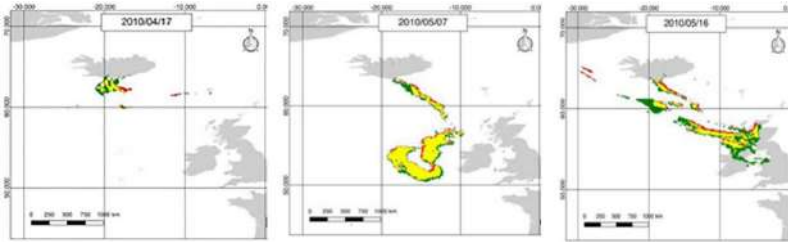
Fig. 4.98. Comparative analysis of various monitoring techniques of volcanic dust distribution as a result of Eyjaföll eruption: dust cloud detected using two methods (yellow color), data delivered by SEVIRI sensor (red color) and DDA AIRS data (green color) [9]
