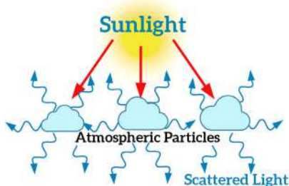
Fig.2.5. Scattering of light [5]
