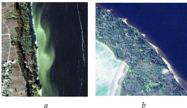
Fig. 4.33. Examples of abrasive banks in Kyiv Region on satellite images of the Google Earth ( a — in the north of Rzhyshchiv Urban-Type Settlement (Kaharlytskyi District); b — in the west of Vytachiv Village (Obukhivskyi District)).
