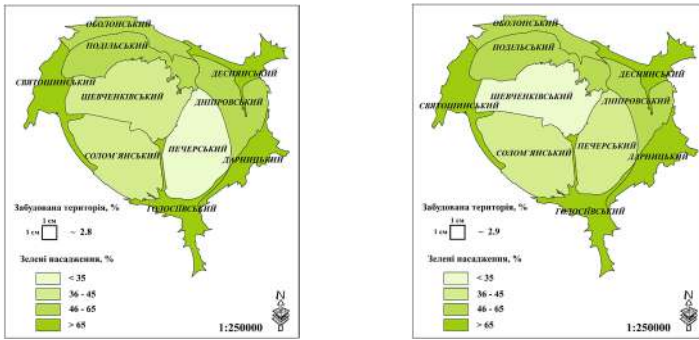
Fig. 4.54. Anamorphic maps of green areas distribution across the districts of Kyiv city, as of: a) 11.07.1989, b) 06.08.2013
