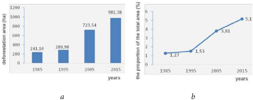
Fig. 4.69. The dynamics of deforestation within the boundaries of the Boiarska Forest Research Station in 1985–2015: a ) the area of deforestation (ha); b ) share of the total area (%) [13].
